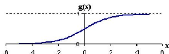
Figure 5. sigmoid function
