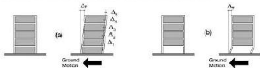
Figure 2.2 Distribution of total displacement generated by an earthquake in: (a) a regular building; and (b) a building with soft story irregularity.
