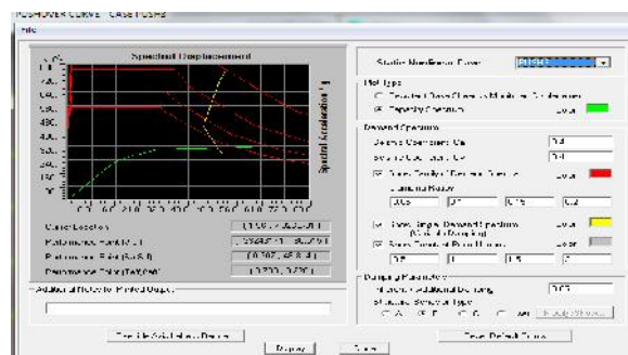
Figure: Performance point of twelve storied building Model 1 along transverse direction
