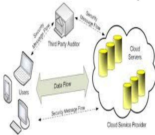
Figure 1: Architecture of Authorized Deduplication
