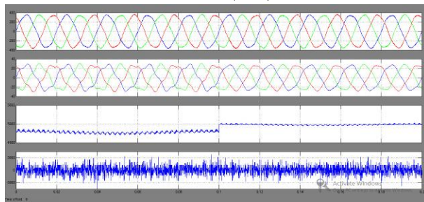
Fig.18. Three Phase Output Voltages(Vabc) And Currents(Iabc)
