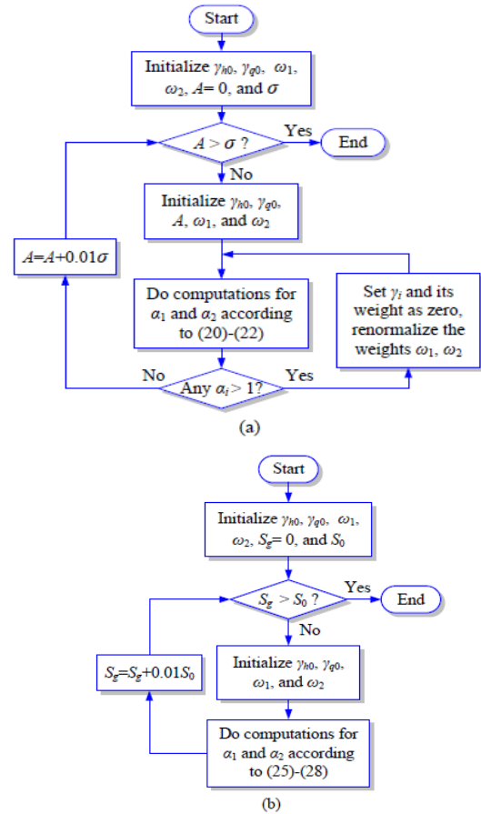
Fig. 7. Flowcharts to solve the optimal compensation model of the MFGTI according to (a) objective I for A \in [0, \sigma] and (b) objective II for S_g \in [0, S_0] .
