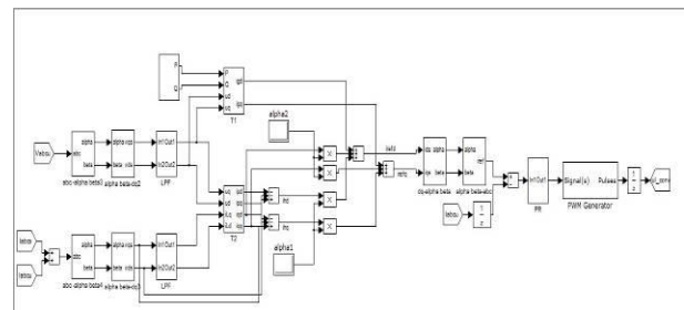
Fig.10. svpwm controller for generation of gate pulses
