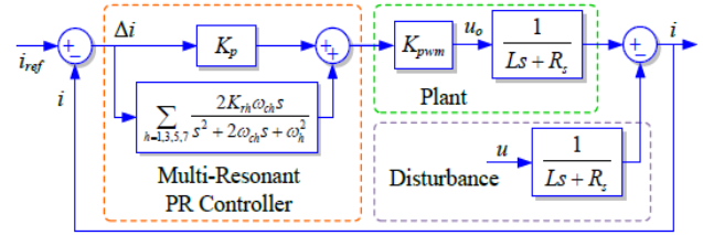
Fig.4. Control block diagram of the MFGTI.
