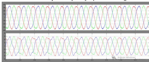
Fig.20. Three Phase Output Voltages(Vabc) And Currents(Iabc)
