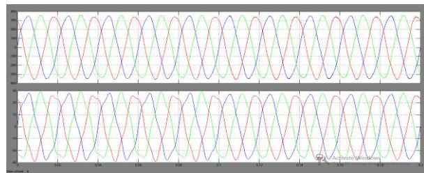
Fig.30. Three Phase Output Voltages(Vabc) And Currents(Iabc)
