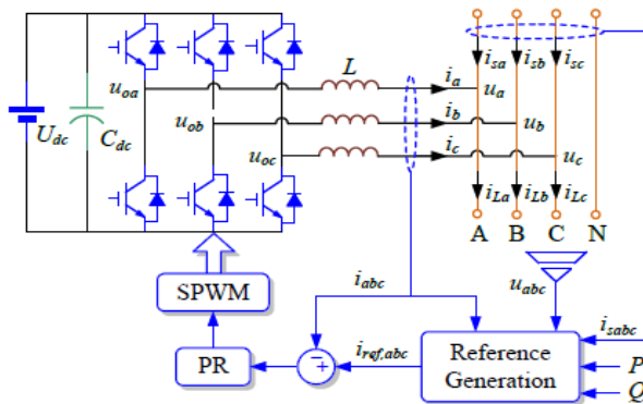
Fig.3. Topology and the overview control strategy of the MFGTI.
