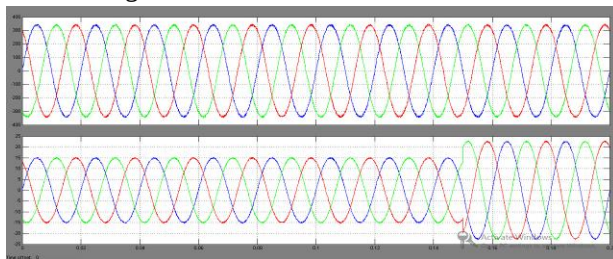
Fig. 15. Three Phase Output Voltages(Vabc) And Currents(Iabc)
