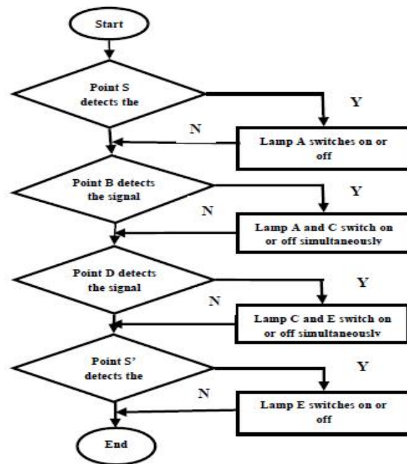
Fig: The control flow chart MICROCONTROLLER:
