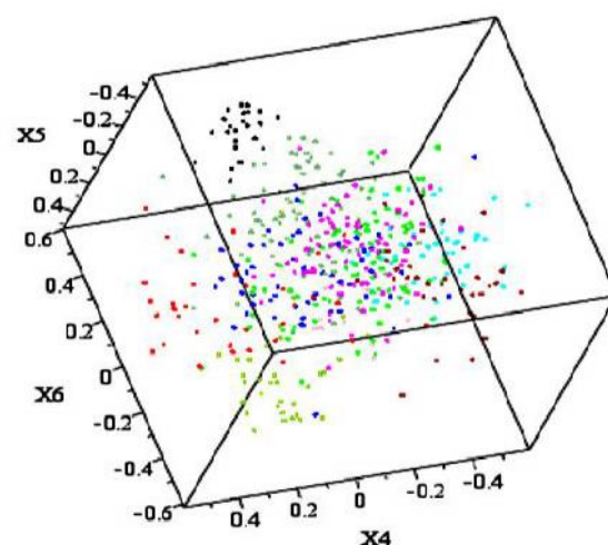
Fig.1.Graph model
