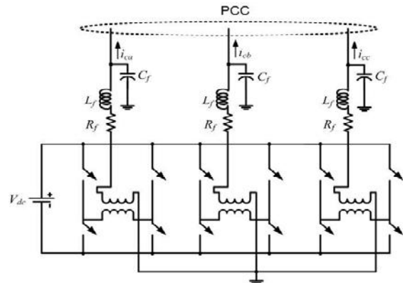
Fig.3: Three-phase converter structure for the compensator
