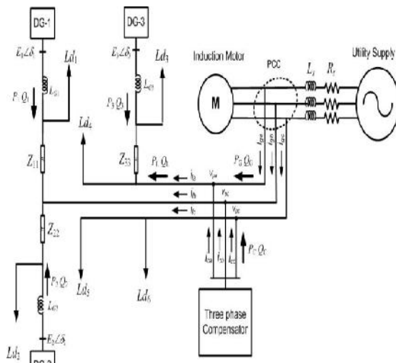
Fig.1: Structure of the grid system under consideration
