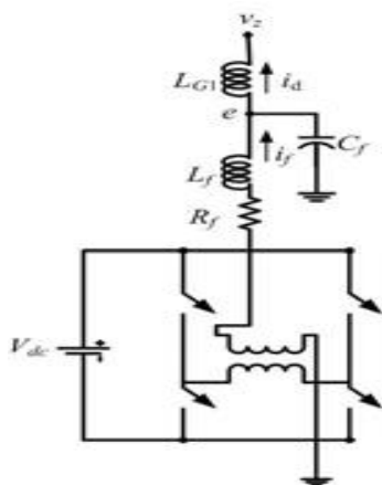
Fig.1: Structure of the grid system under consideration
