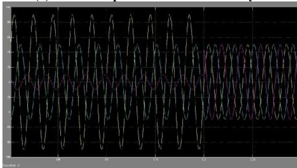
(b) Three phase compensator current
