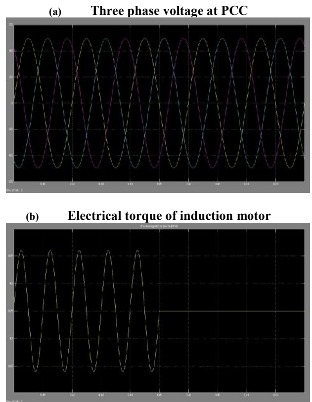
Fig.13: Voltage at PCC and induction motor torque
