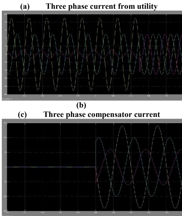
Fig.11: Three phase current from utility and DG-compensator
