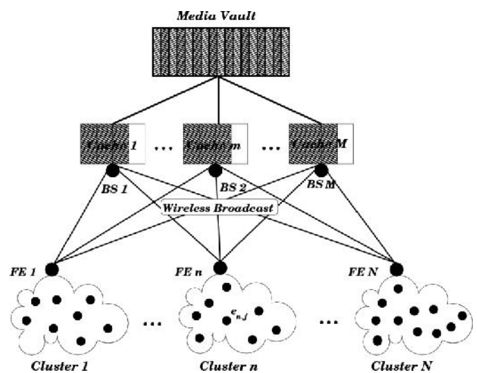
Fig. 1: Wireless content distribution. A media vault is used to place content in caches at wireless BSs, which can
