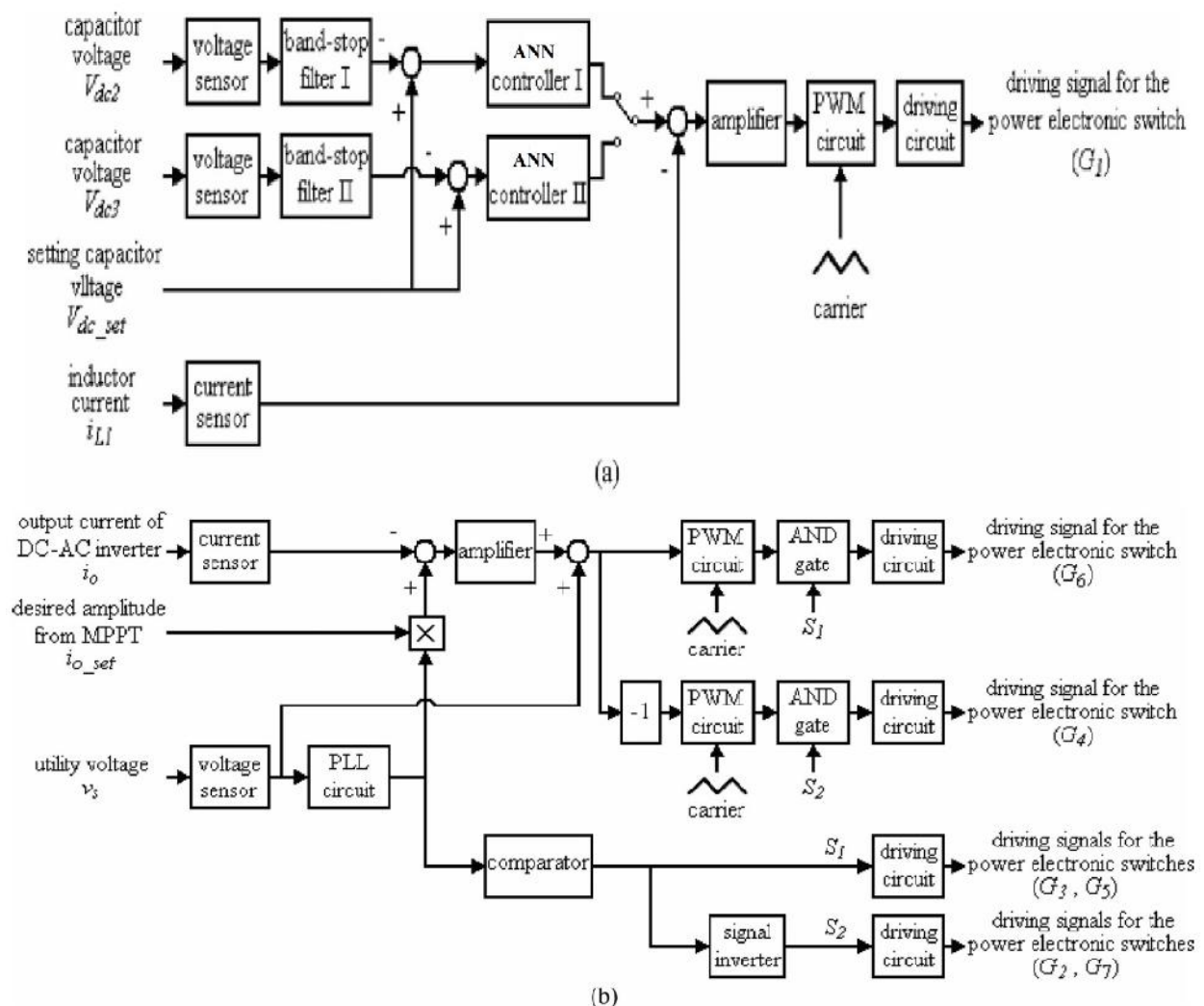
Fig. 11. Control block of the proposed transformer less grid- connected ANN based power converter. (a) DC–DC power converter. (b) DC–AC inverter.
