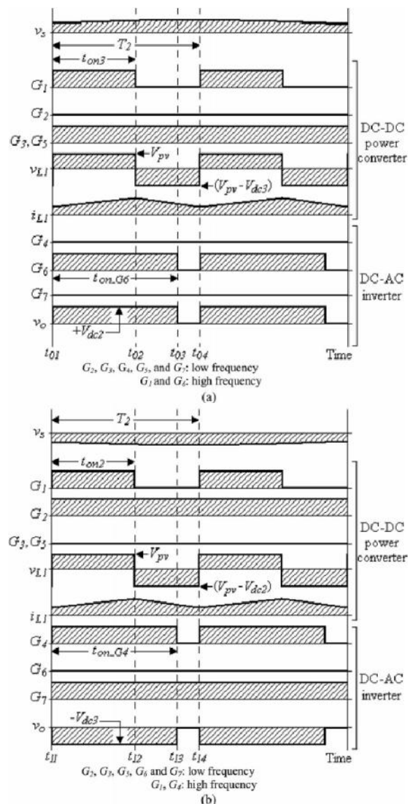
Fig. 7. Timing sequence for power electronic switches of the proposed power converter. (a) Positive half-cycle. G2 , G3, G4 , G5, and G7 : low frequency, G1 and G6 : high frequency. (b) Negative half-cycle. G2 , G3 , G5 , G6 and G7 : low frequency, G1 , G4 : high frequency.
