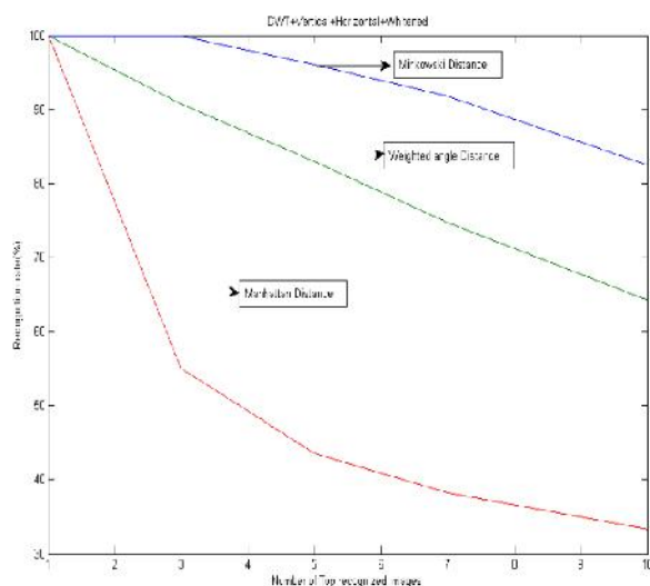
Figure 4. Comparative recognition rates.
