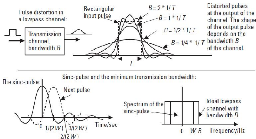
Figure 3 Symbol rate (baud rate) and bandwidth.
