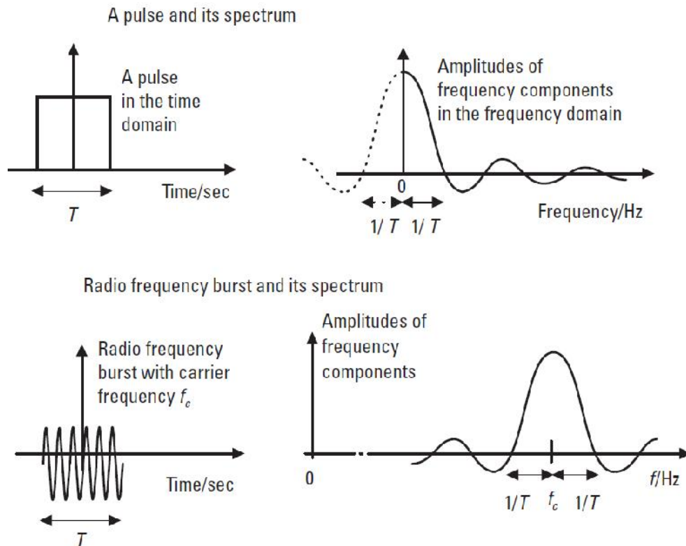
Figure .7 Spectrum of the pulse from low frequencies to carrier frequencies
