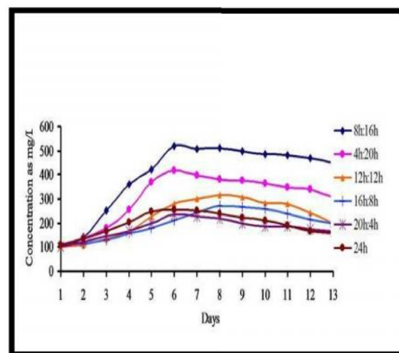
Fig1: Biomass growth patterns of C.vulgaris at different light/dark cycles grown in shake flasks.
