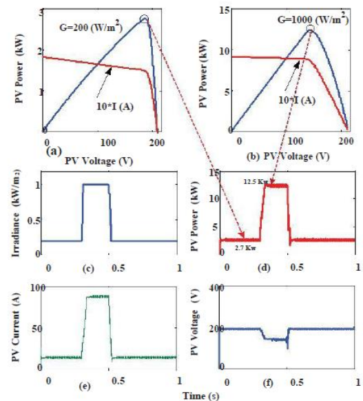
Fig. 6. MPPT Tracking performance of HGICB Converter (a) PV Characteristic at G=200 \text{ W/m}^2 (b) PV Characteristic at G=1000 \text{ W/m}^2 (c) insolation variations (d) PV Maximum Power (e) PV Current (f) PV Voltage.
