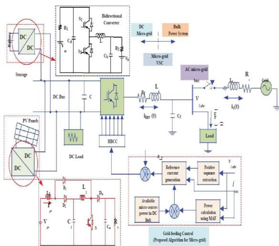
Fig. 1. Proposed HECS model
