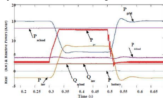
Fig. 8. Real and Reactive Power flow waveforms of PV hybrid generating system.
