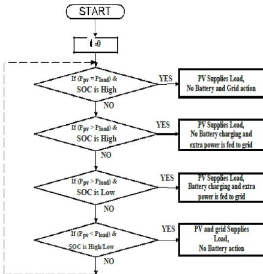
Fig. 3. Hybrid system flow chart of power flow
