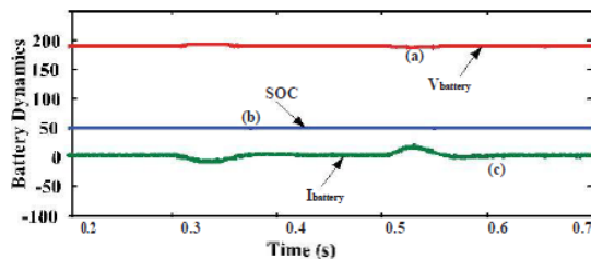
Fig. 11. Battery performance using proposed control approach to bidirectional battery converter: (a) Battery Voltage (b) State of charge (SOC) (c) Battery current.
