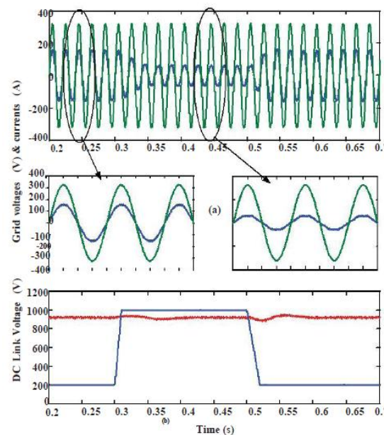
Fig. 9. Simulation results: performance of proposed control approach (a) Grid Voltages and currents (b) Dc Link Voltage Dynamics with different insolation
