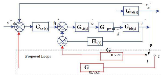
Fig. 4. Inner and outer loops of battery converter
