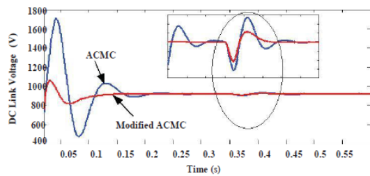
Fig. 10. DC Link Voltage Dynamics using ACMC and MACMC Control algorithms
