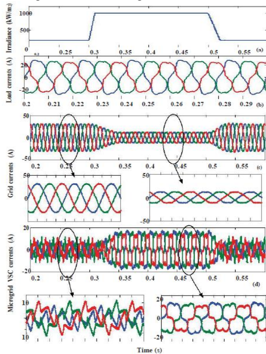
Fig. 7. Performance of proposed control approach for Micro-grid side VSC: (a) Insolation Changes (b) Load currents (c) Grid currents (d) \mu G-VSC currents.
