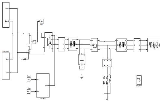
Fig. 5. Simulink model of proposed HECS
