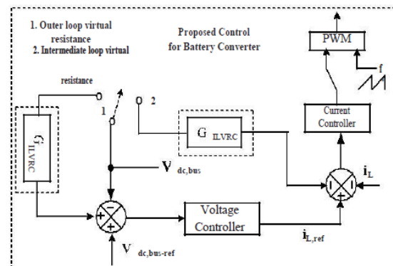
Fig. 2. Advanced ACMC control strategy for battery converter
