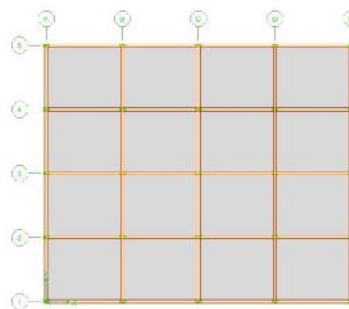
Figure 4.1 b: Plan of Model -2 (Stiffness of walls considered)
