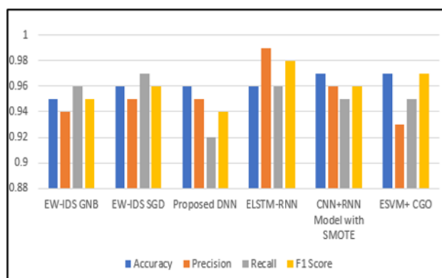
Fig 1. Comparison Graph of different Algorithms
